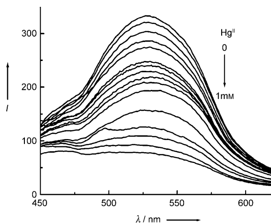
Figure 1. Fluorescence spectra of 1 ( 48 \mu\text{g mL}^{-1} ) with increasing concentration of \text{Hg}^{\text{II}} ions in aqueous solution containing 4% \text{CH}_3\text{CN} ( \lambda_{\text{ex}} = 330 \text{ nm} ).
