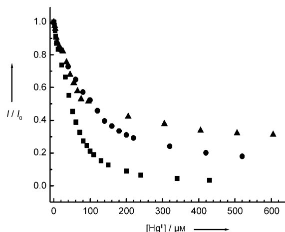
Figure 4. Titration of 3 ( \blacksquare , 1.0 \times 10^{-5} \text{ M} ), 2 ( \bullet , 1.0 \times 10^{-5} \text{ M} ), and 1 ( \blacktriangle , 48 \mu\text{g mL}^{-1} ) with \text{Hg}^{\text{II}} in aqueous solution containing 4% \text{CH}_3\text{CN} ( \lambda_{\text{ex}} = 330 \text{ nm} ).
