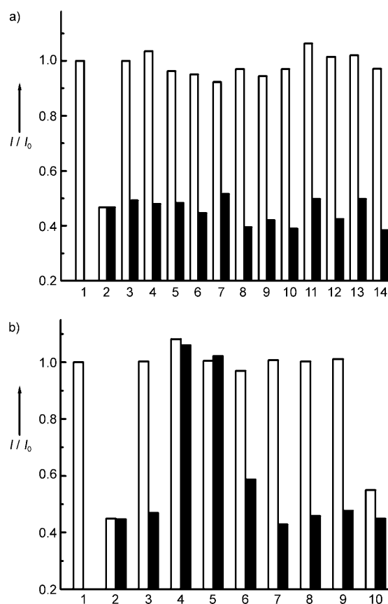
Figure 2. Relative fluorescence intensity of 1 ( 48 \mu\text{g mL}^{-1} ) in the presence of various interfering ions (2 mM, white bars) and coexistence (black bars) of interfering ions (2 mM) with \text{Hg}^{\text{II}} (0.2 mM), in 4% \text{CH}_3\text{CN} aqueous solution ( \lambda_{\text{ex}} = 330 \text{ nm} ). Interfering ions containing a) metal ions [1] no ions, 2) \text{Hg}^{\text{II}} , 3) \text{Zn}^{\text{II}} , 4) \text{Cd}^{\text{II}} , 5) \text{Fe}^{\text{II}} , 6) \text{Co}^{\text{II}} , 7) \text{Ni}^{\text{II}} , 8) \text{Pb}^{\text{II}} , 9) \text{Cu}^{\text{II}} , 10) \text{Ag}^{\text{I}} , 11) \text{K}^+ , 12) \text{Ca}^{2+} , 13) \text{Na}^+ , 14) \text{Mg}^{2+} ; b) anions [1] none, 2) \text{Hg}^{\text{II}} , 3) \text{F}^- , 4) \text{Cl}^- , 5) \text{Br}^- , 6) \text{I}^- , 7) \text{H}_2\text{PO}_4^- , 8) \text{NO}_3^- , 9) \text{AcO}^- , 10) \text{HSO}_4^- .
