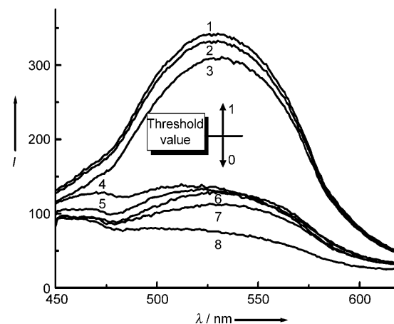
Figure 3. Fluorescence spectra of 1 ( 48 \mu\text{g mL}^{-1} ) under different input conditions. 1) ( 1 + \text{Cl}^- ), 2) 1 , 3) ( 1 + \text{Hg}^{\text{II}} + \text{Cl}^- ), 4) ( 1 + \text{Hg}^{\text{II}} ), 5) ( 1 + \text{H}^+ ), 6) ( 1 + \text{Cl}^- + \text{H}^+ ), 7) ( 1 + \text{Hg}^{\text{II}} + \text{Cl}^- + \text{H}^+ ), and 8) ( 1 + \text{Hg}^{\text{II}} + \text{H}^+ ). Fluorescence intensities higher than the threshold value specified at 530 nm are assigned as 1 and intensities lower than that value are assigned as 0.
