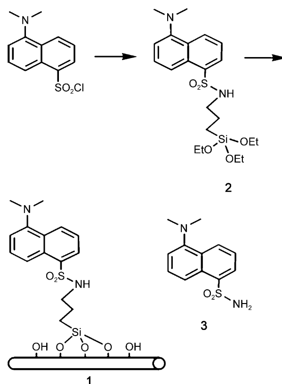
Scheme 1. The structures of the functional molecules and the SiNW modification procedure.
